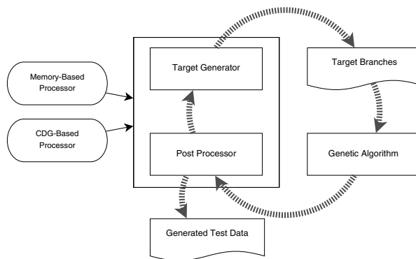
Fig. 5. Flowchart of the memory-based approach and the CDG-based approach.
