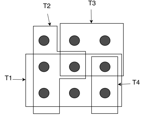
Fig. 2. An example of greedy algorithm for set cover problem. Here, a program consists of 9 branches and T = T_1, T_2, T_3, T_4 . The greedy algorithm produces set cover of size 3 by selecting the test data: T_1, T_3 and T_2 in this order.
